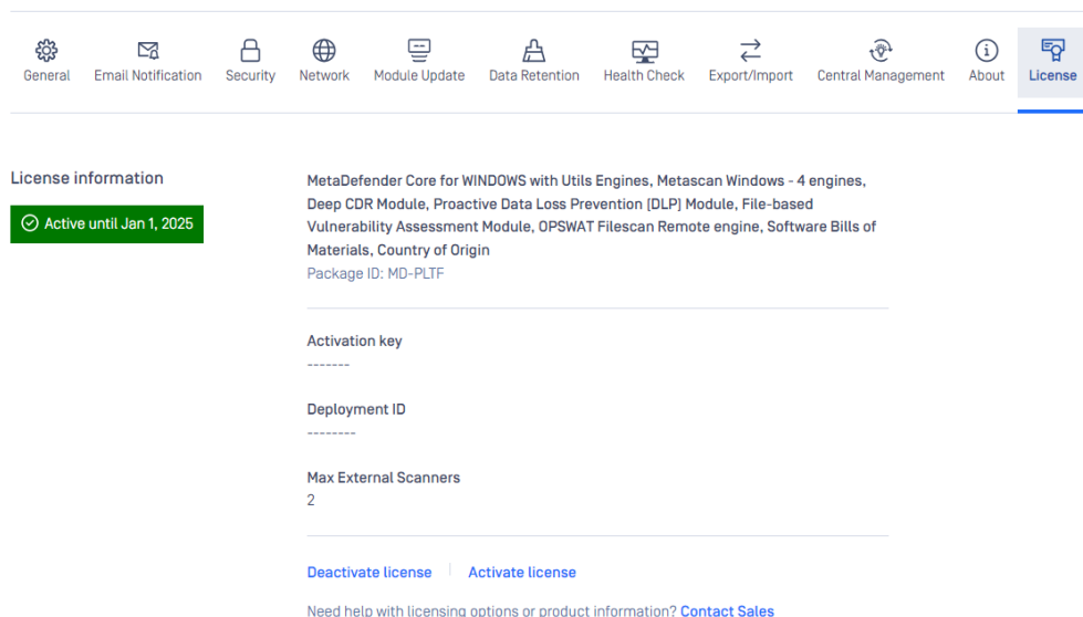
Figure 24 – License information
