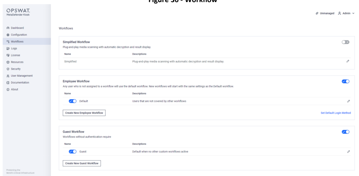
Figure 36 - Workflow
